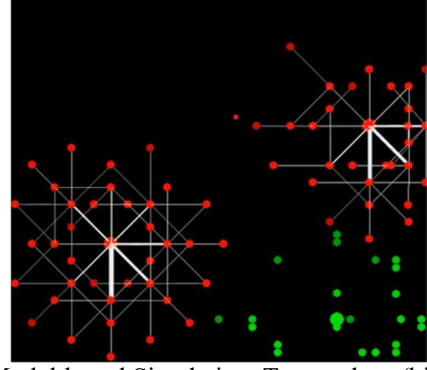
Figure 4: Model-based Simulation. Two wolves (big red circles) pursuing a single sheep (big green circles) at single time step. The model simulates multiple futures, going several steps into each. Smaller red and green circles indicate possible future locations for the agents. The line thickness and circle shade indicate how often a given action has been taken in simulation. The best action is the one taken most frequently.
